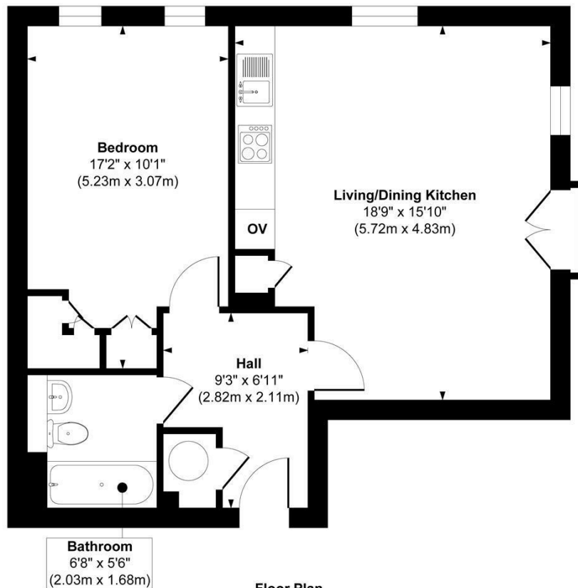
Floor Plan
